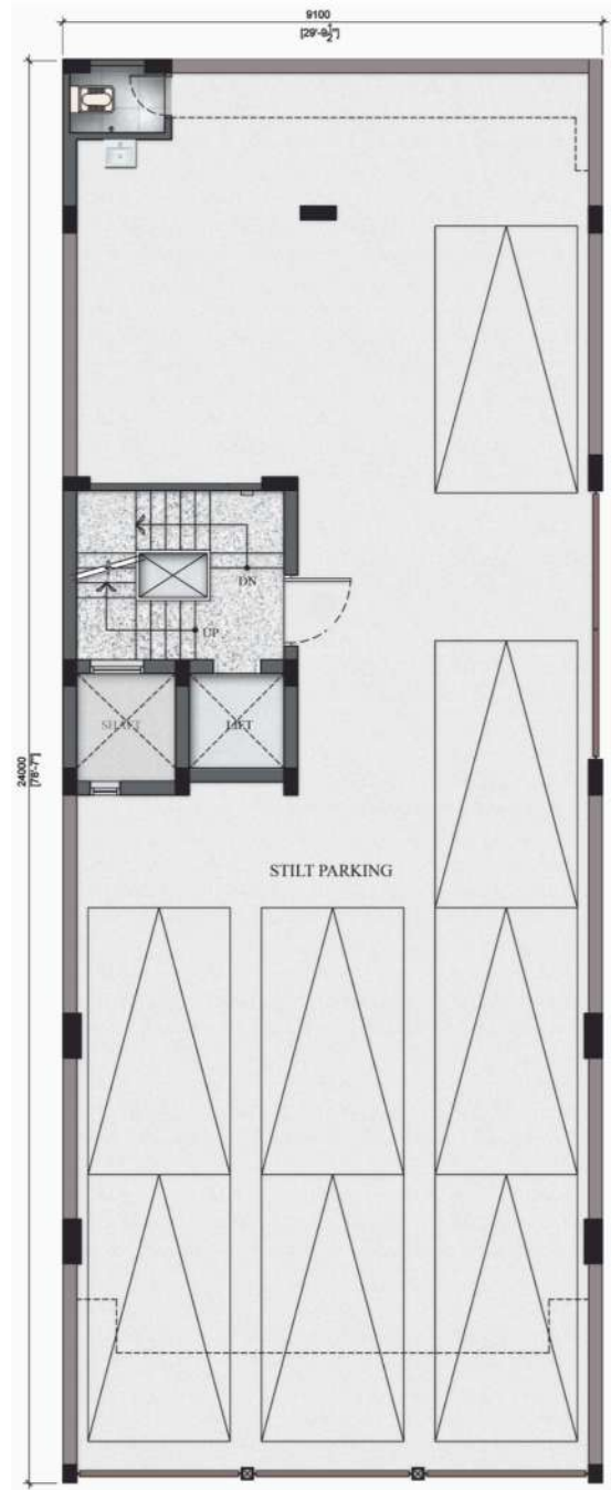
Stilt Plan
